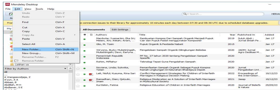
Gambar 2. Mendelay Desktop
